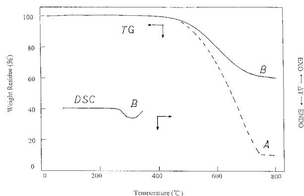
Figure 1 TGA and the second heating DSC curves for PAI IIIj with a heating rate of 20°C min -1 . (---) In air. (—) In nitrogen.
