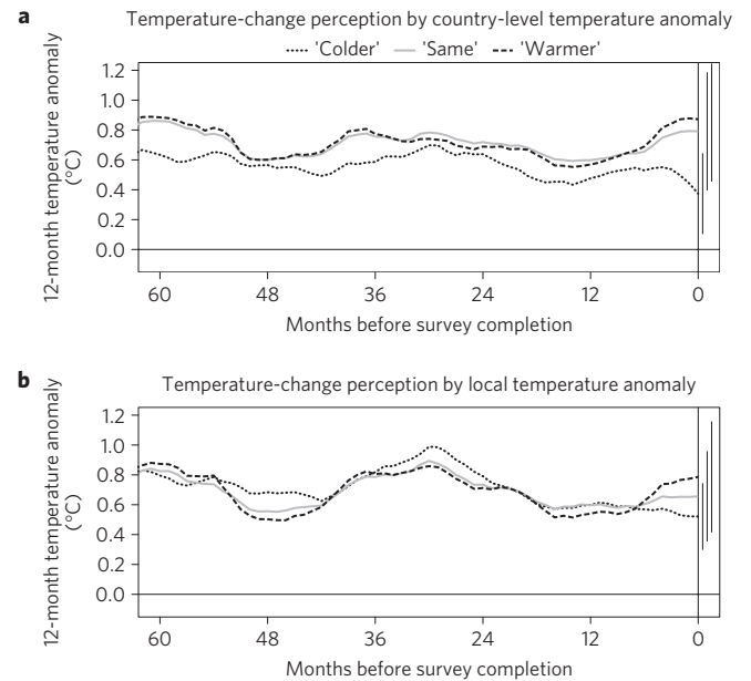
Figure 1 | Time series of mean temperature anomaly by response to 5-year temperature-change perception item. The vertical axis represents the population-weighted 12-month running mean temperature anomaly (departure from 1961 to 1990 mean). The horizontal axis represents months before the survey completion date. The vertical bars represent standard deviations. a , National population-weighted temperature anomalies (89 countries). b , Subnational population-weighted temperature anomalies (46 countries, 433 regions).
