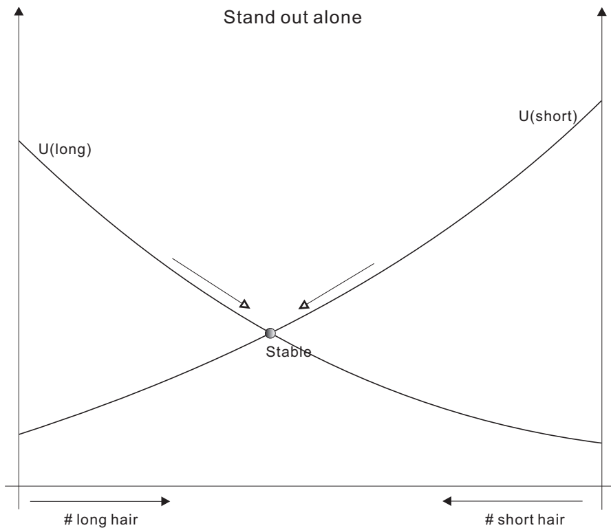
Figure 4: Network externality
