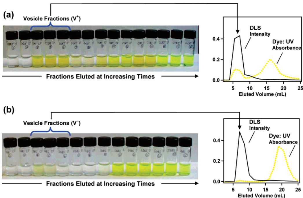
Figure 2. Results from SEC of vesicles with the anionic dye CF: (a) V^+ vesicles and (b) V^- vesicles. The plots on the right show the DLS intensity, which is proportional to vesicle concentration, and the UV absorbance at 492 nm, which is proportional to CF concentration, as a function of eluted volume. The results show that a significant portion of the dye (23%) elutes with the V^+ vesicles, whereas only about 1.5% of the dye elutes with the V^- vesicles. This can be seen visually by the more intense yellowish hue of the vesicle fractions (vials 3–5) in the V^+ case.
