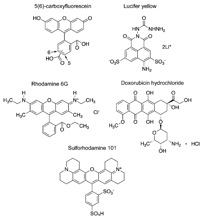
Figure 1. Structures of the five solutes used in these studies.
