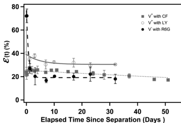
Figure 3. Dye release profiles. An evaluation of long-term release was achieved by monitoring \epsilon as a function of time. Data were acquired for CF (■) and LY (○) in V^+ samples and R6G (●) in V^- samples. The corresponding lines are fits to an exponential decay. For CF in V^+ , three trials were completed, and the error bars on the points are the standard deviations of the averages of the three data sets. For R6G and LY, two trials were run, and the error bars are the actual values for the two trials.
