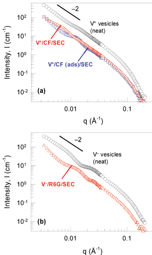
Figure 5. SANS data for neat and dye-containing V^+ and V^- samples. (a) Scattering data for V^+ samples. A -2 slope characteristic of bilayer scattering is observed for neat vesicles ( \circ ) and when CF is added before ( \Delta ) or after ( \square ) vesicles are formed. (b) Scattering data for neat V^- samples ( \circ ) and for V^- loaded with R6G ( \Delta ). As in plot a, the data from both samples are consistent with the presence of vesicles. The neat vesicle samples ( \circ ) were run as-prepared with 1% total surfactant concentration. The other samples ( \square , \Delta ) were diluted by approximately 4-fold as a result of undergoing SEC.
