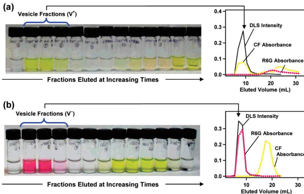
Figure 4. Vesicle-mediated separation of mixtures of R6G and CF dyes using (a) V^+ vesicles and (b) V^- vesicles. The plots on the right show the DLS intensity, which is proportional to vesicle concentration, and the UV absorbances, which are proportional to the concentrations of R6G and CF, as a function of eluted volume. The results show that the V^+ vesicle fractions contain 31% of the initial amount of CF with no detectable R6G whereas the V^- vesicle fractions contain 88% of the initial amount of R6G with no detectable CF. This can be seen visually by the yellowish hue of the V^+ vesicle fractions compared to the pinkish hue of the V^- vesicle fractions.
