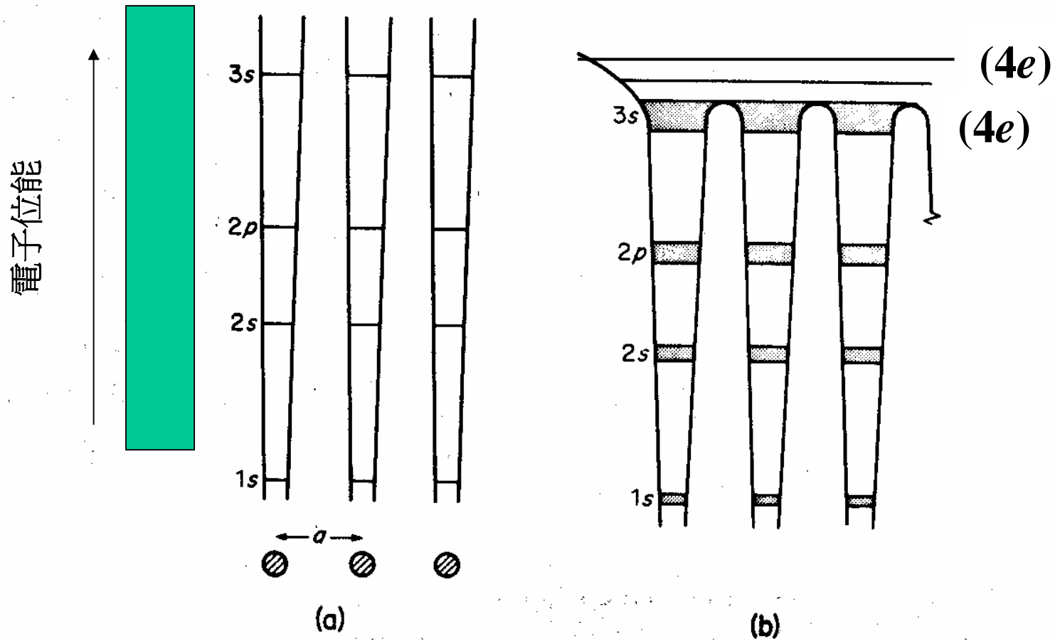
FIG. 18.29 Energy levels in sodium: (a) isolated atoms; (b) section of crystal. The sharp levels in the atom have become bands in the crystal.
