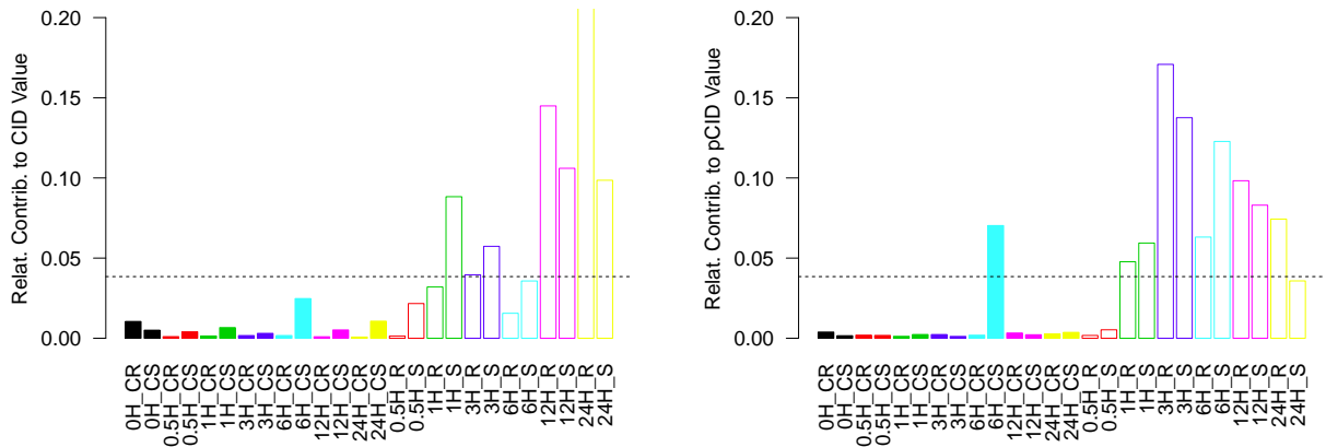
Figure S2. Expression profiles and CID/pCID inferences of 253114_at based on expression levels of CBF1 and CBF3 . (A) Averages and standard deviations of log2 expression levels over time under control (CTRL) or cold treatments. (B) Contribution to CID(253114_at| CBF1 ) (left) and pCID(253114_at| CBF3 ; CBF1 ) (right) by different sub-samples. C: control; S: shoot; R: root. The dashed horizontal line indicates the nominal value 1/26.
