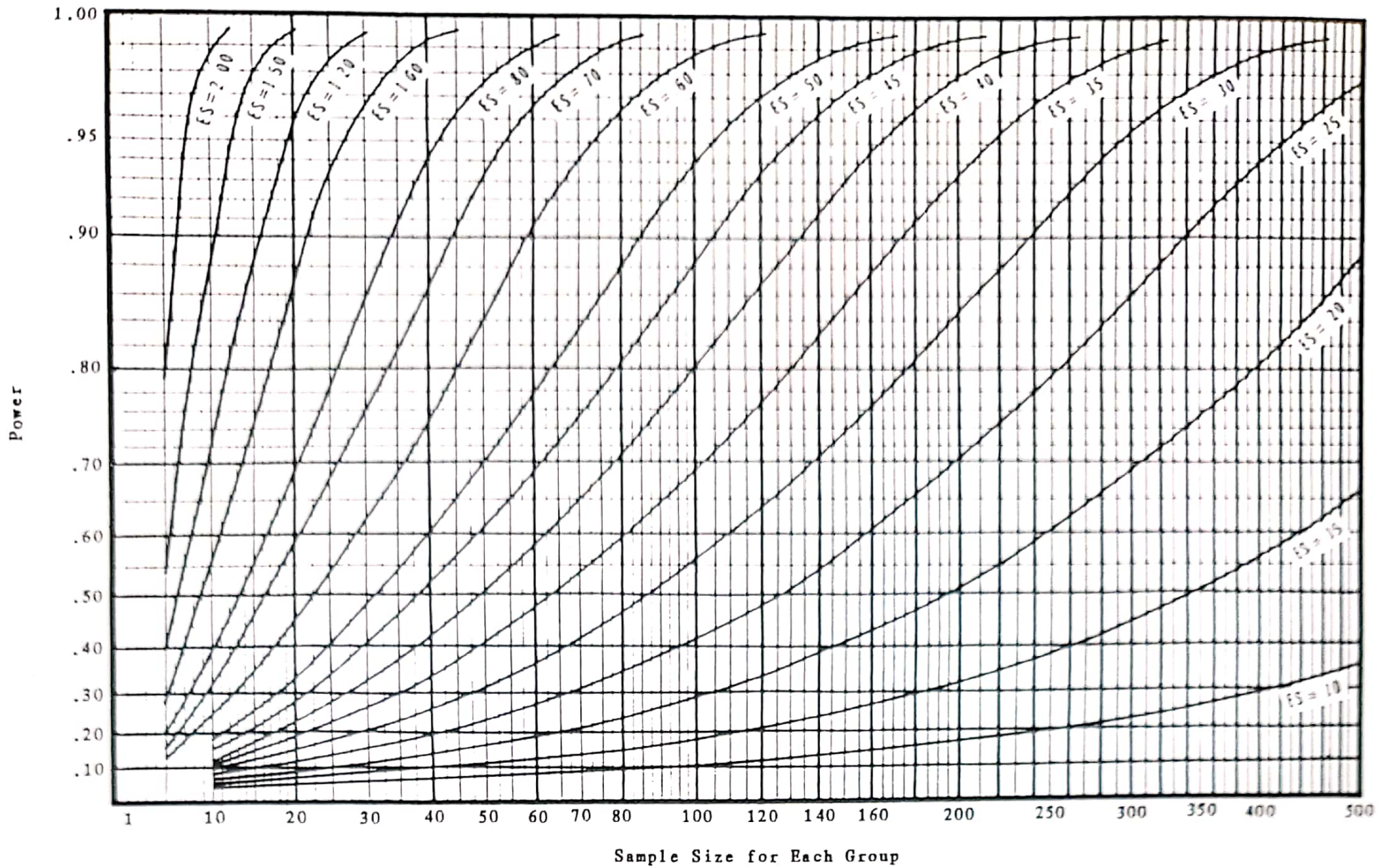
Figure 4.4: Power Chart for \alpha = .05 , Two-Tailed or \alpha = .025 , One-Tailed
