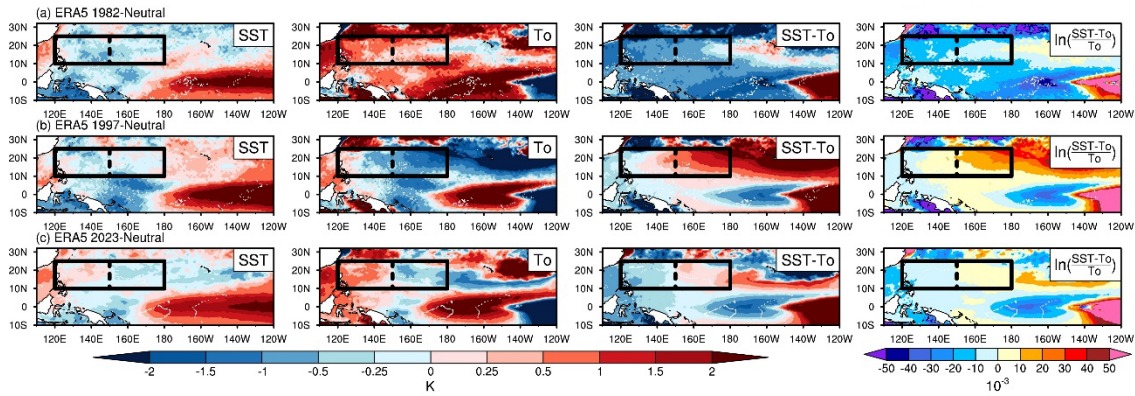
Figure S1. Spatial distribution of SST, T_o , SST-T_o , and efficiency \ln\left(\frac{SST-T_o}{T_o}\right) terms for (a) 1982, (b) 1997, and (c) 2023 EP El Niño minus neutral ENSO from ERA5. The black boxes indicate the MDR. The 150°E longitude denoted by the dashed line divides the MDR box into two areas. The spatial resolution of ERA5 is 0.25°.
