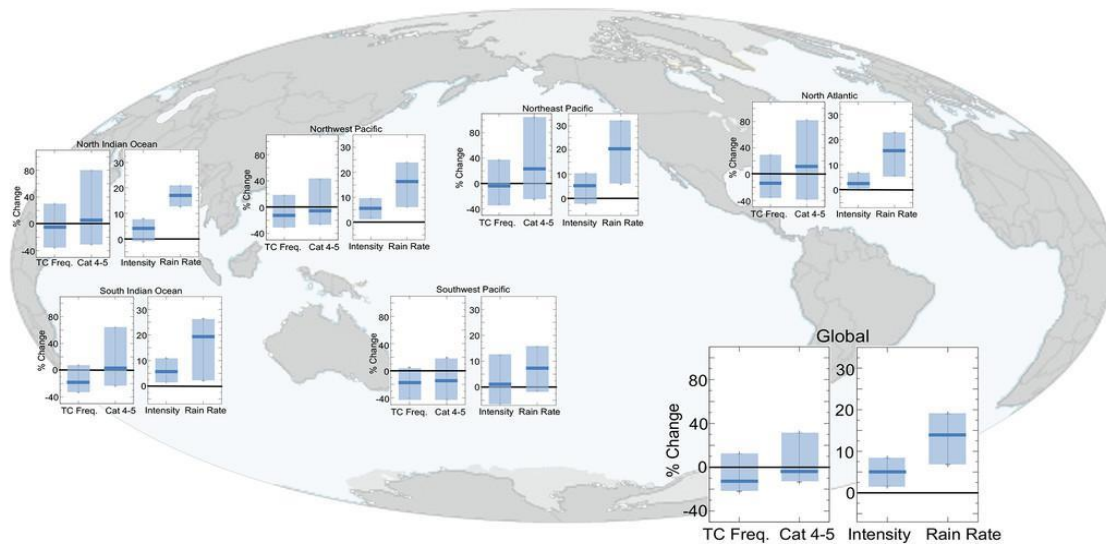
Figure 6.3.3: Summary of TC projections for a 2°C global anthropogenic warming. Shown for each basin and the globe are median and percentile ranges for projected percentage changes in TC frequency, Cat. 4–5 TC frequency, TC intensity, and TC near-storm rain rate. For TC frequency, the 5th–95th-percentile range across published estimates is shown. For Cat. 4–5, TC frequency, TC intensity, and TC near-storm rain rates the 10th–90th-percentile range is shown. Adapted from Knutson et al. (2020).
