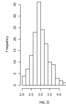
Histogram of iris[, 2]
