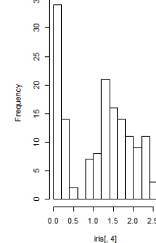
Histogram of iris[, 4]
