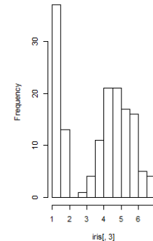
Histogram of iris[, 3]
