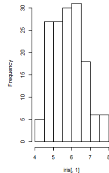
Histogram of iris[, 1]
