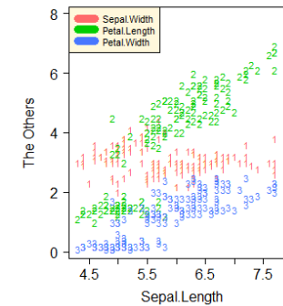
gth vs Sepal.Width, Petal.Length,
