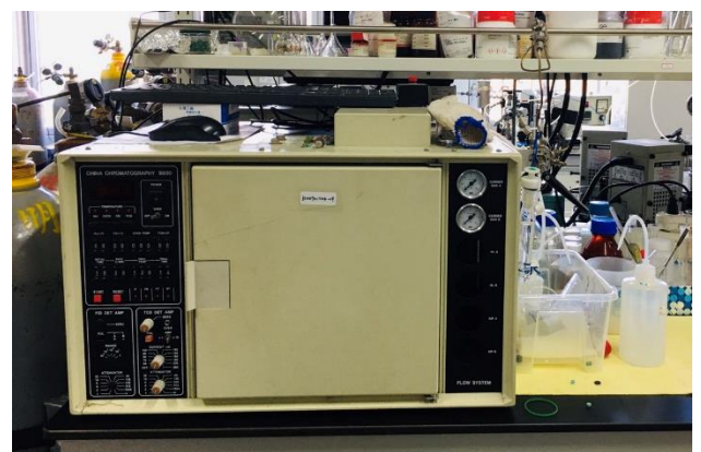
氣相層析儀(GC)(CHINA CHROMATOGRAPHY 9800)
