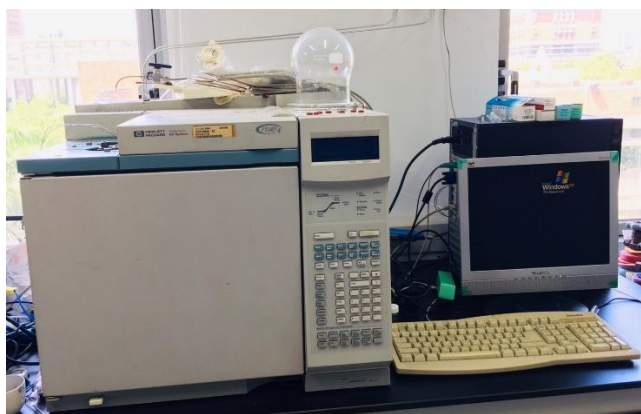
氣相層析儀(GC)(HP 6890 Series)
