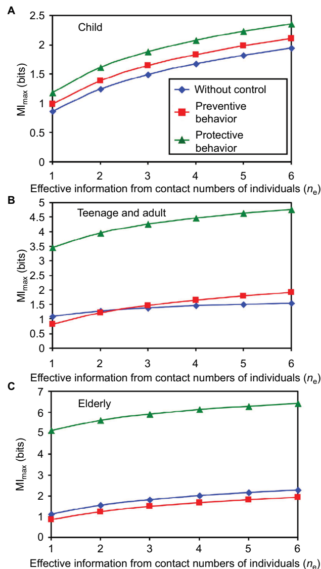
Figure 4 MI_{max} estimates with/without control and preventive and protective behaviors for (A) child, (B) teenage and adult, and (C) elderly age groups, respectively. Abbreviations: n_e ; effective information from contact numbers of individuals; MI_{max} , maximum mutual risk perception information.
