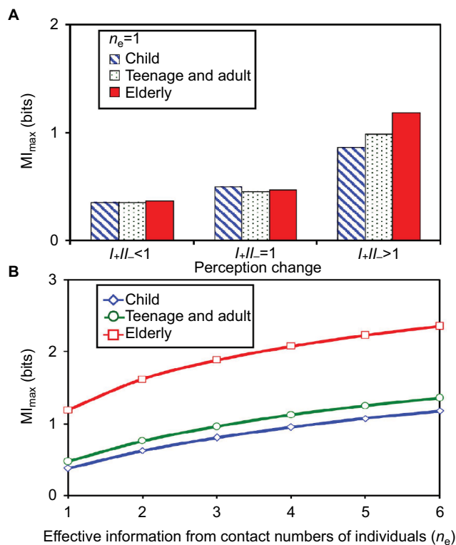
Figure 3 Age-specific MI_{max} estimates (A) for perception change with different overlapping percentage scenarios at contact numbers of individuals, n_e = 1 , and (B) based on network-based information model varied with n_e . Abbreviations: MI_{max} , maximum mutual risk perception information.
