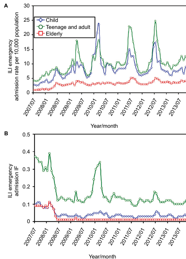
Figure 1 ILI-related emergency admission rates and IF among the three age groups, child (0–14 years), teenage and adult (15–64 years), and elderly (>65 years), in Taiwan. Note: (A) ILI-related emergency admission rate, and (B) ILI-related emergency admission IF. Abbreviations: ILI, influenza-like illness; IF, infection fraction.
