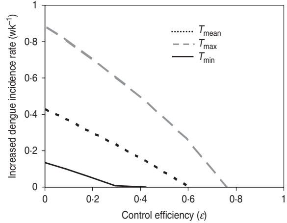
Fig. 6. Relationship between weekly increased dengue incidence rate ( wk^{-1} ) and the control efficiency varied according to T_{min} , T_{mean} , and T_{max} .
