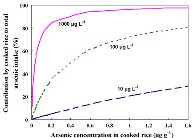
Fig. 6. The PBPK model predicted percentage contributions of cooked rice to daily arsenic intake varied with arsenic contents in drinking water of 10, 100, and 1000 µg L -1 .
