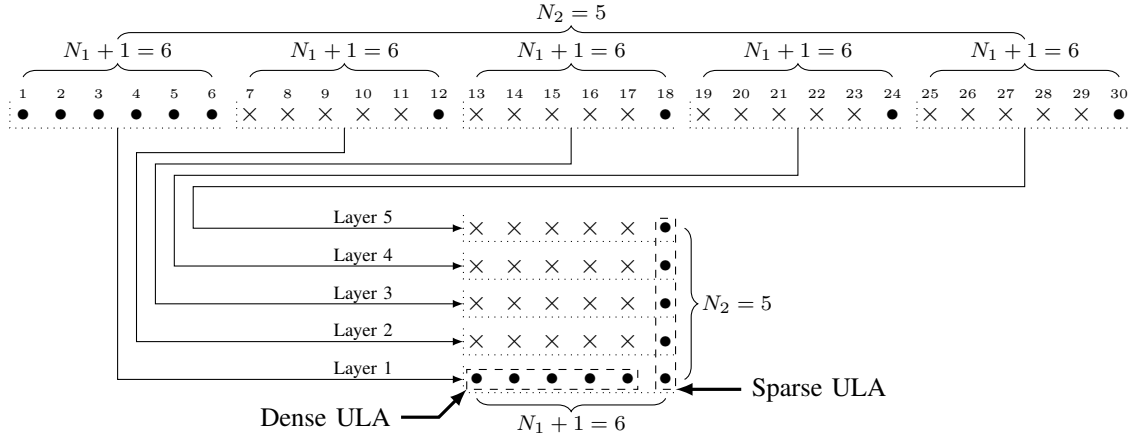
Fig. 1. The concept of 2D representations of linear arrays. The top of this figure shows the 1D representation of a nested array with N_1 = N_2 = 5 , where bullets denote sensors and crosses indicate empty locations. In the 1D representation of this example, the array aperture is divided into N_2 = 5 layers of size N_1 + 1 = 6 . These layers are stacked into the associated 2D representation, as marked by arrows. Notice that in this paper, 2D representations denote linear arrays, not planar arrays . They are introduced to simplify the discussion in the future development.
