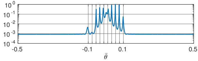
(c) Nested array, D = 10 , E = 0.01216 .
