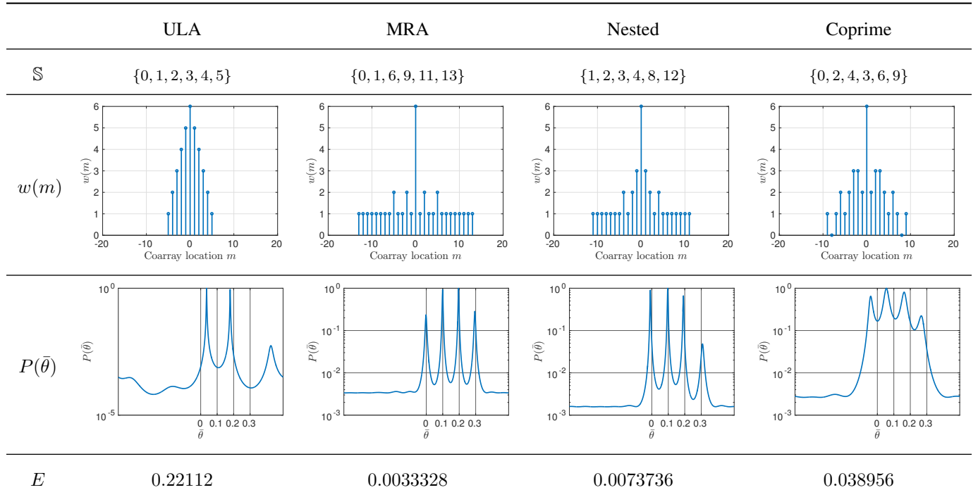
Fig. 4. Comparison among ULAs, MRAs, nested arrays, coprime arrays and their MUSIC spectra P(\bar{\theta}) in the presence of mutual coupling. It can be observed that higher uniform DOF and smaller weight functions w(1) , w(2) , w(3) tend to decrease the RMSE.
