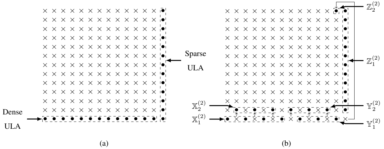
Fig. 6. 2D representations of (a) the parent nested array, and (b) the corresponding second-order super nested array, \mathbb{S}^{(2)} , where N_1 = N_2 = 13 . Bullets denote sensor locations while crosses indicate empty locations. Thin arrows illustrate how sensors migrate from nested arrays to second-order super nested arrays. The dense ULA in nested arrays is split into four sets: \mathbb{X}_1^{(2)} , \mathbb{Y}_1^{(2)} , \mathbb{X}_2^{(2)} , and \mathbb{Y}_2^{(2)} in second-order super nested arrays. The sensor located at N_1 + 1 , belonging to the sparse ULA of nested arrays, is moved to location N_2(N_1 + 1) - 1 in second-order super nested arrays.
