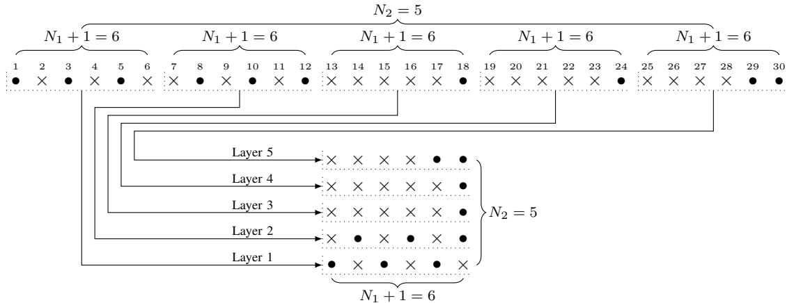
Fig. 2. The 1D and 2D representations of a second-order super nested array with N_1 = N_2 = 5 . It will be proved in this paper that super nested arrays possess the same number of sensors, the same physical aperture, and the same hole-free coarray as their parent nested arrays. Furthermore, super nested arrays alleviate the mutual coupling effect. In this example, there is only one pair of sensors with separation 1, located at 29 and 30. However, for the parent nested array in Fig. 1, locations 1 through 6 are crowded with sensors, leading to more severe mutual coupling effect.
