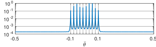
(f) Third-order super nested, D = 10 , E = 0.00023647 .
