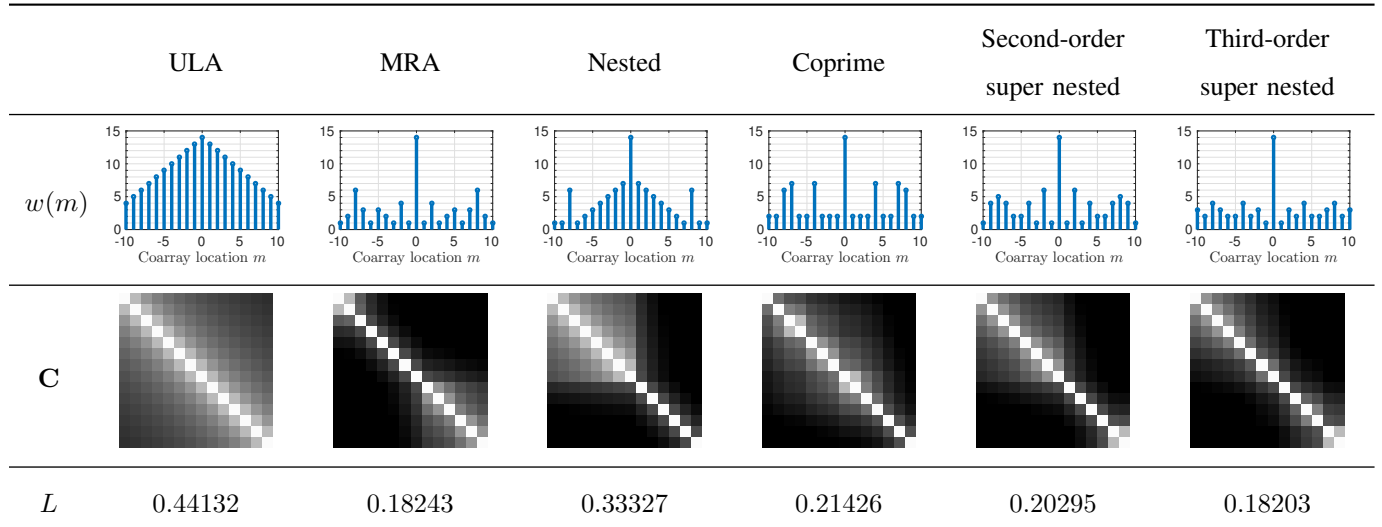
Fig. 7. Comparison among ULA, nested array, coprime array, second-order super nested array, and third-order super nested array in the presence of mutual coupling. The coupling leakage L is defined as \|\mathbf{C} - \text{diag}(\mathbf{C})\|_F / \|\mathbf{C}\|_F , where [\text{diag}(\mathbf{C})]_{i,j} = [\mathbf{C}]_{i,j} \delta_{i,j} .
