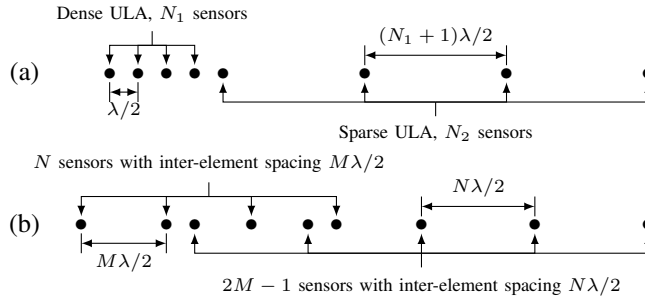
Fig. 3. 1D representations of (a) nested arrays and (b) coprime arrays.
