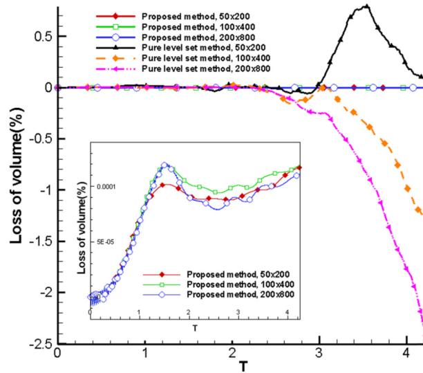
Fig. 13. Comparison of the predicted percentages of the loss of area using different methods under different grid resolutions for the Rayleigh-Taylor instability problem.
