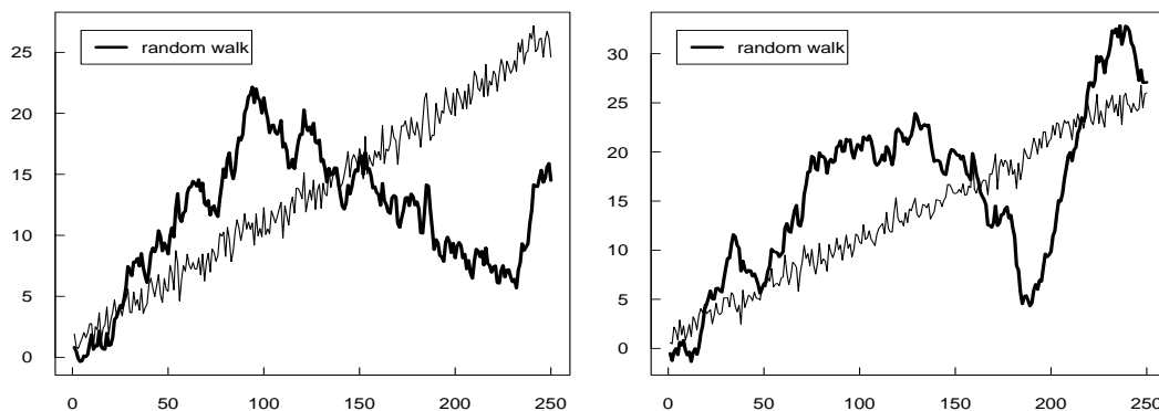
Figure 7.2: Sample paths of random walk and trend stationary series.
