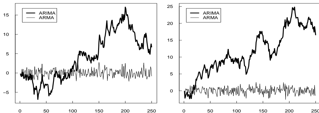
Figure 7.1: Sample paths of ARIMA and ARMA series.
