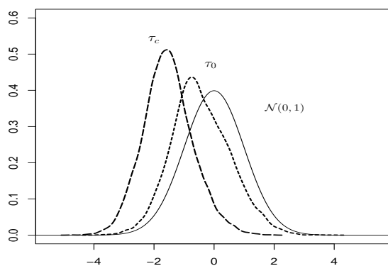
Figure 7.3: The distributions of the Dickey-Fuller tests ( \tau_0 and \tau_c ) vs. \mathcal{N}(0, 1) .
