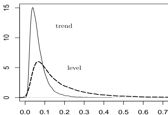
Figure 7.4: The distributions of the KPSS tests.
