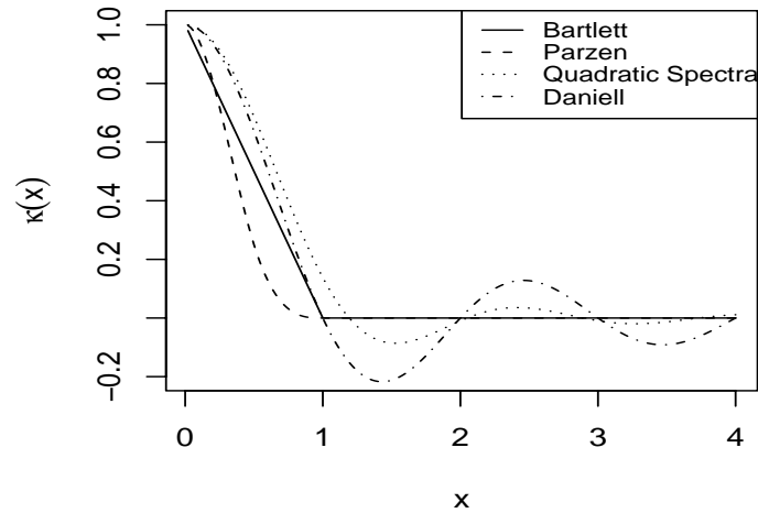
Figure 6.1: The Bartlett, Parzen, quadratic spectral and Daniell kernels.
