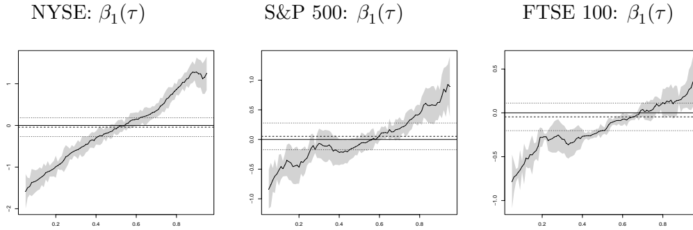
Figure 8: QR and LS estimates of the causal effects of log volume on return: 2000–2006, Model without r_{t-j}^2 .
